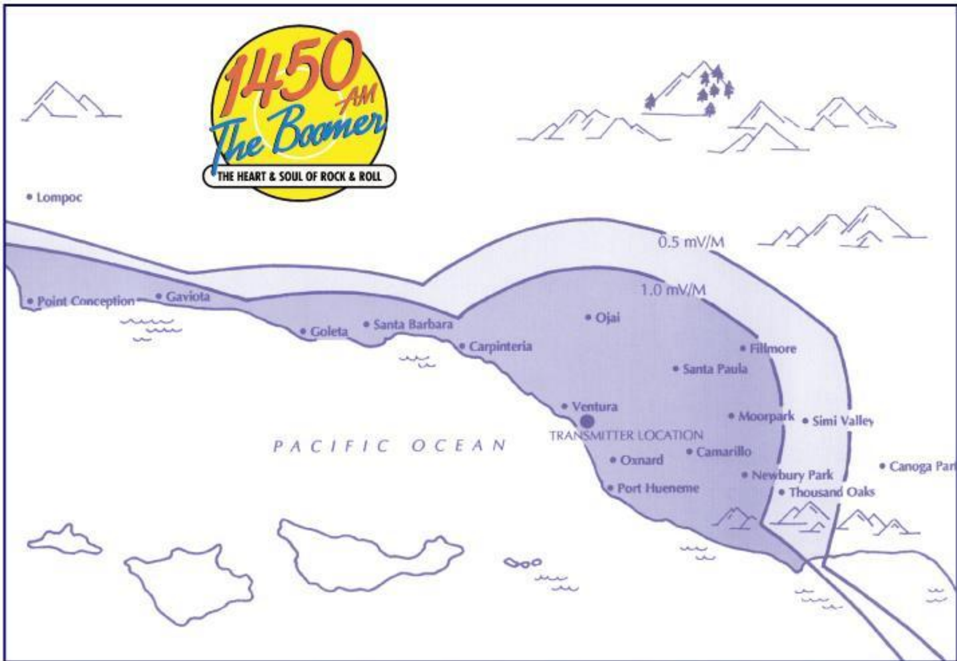
This is an accurate representation of the actual coverage map drawn to FCC Standards by J.D. Strahler, consulting engineer Original on file at KVEN studios.
